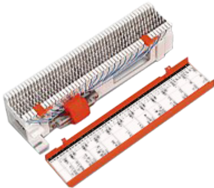
PN#300969 66 Block w/prewired 25pr Amphenol, base, and orange cover
