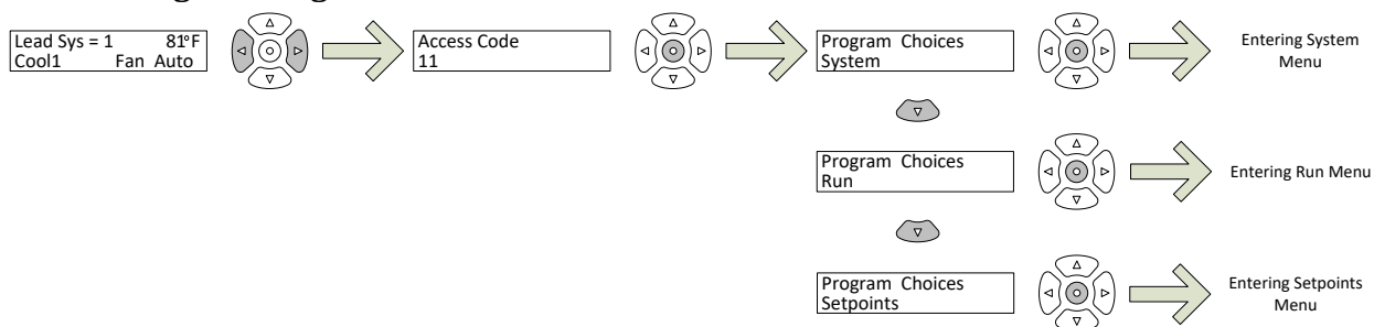
Figure 4 - Programming Flow
